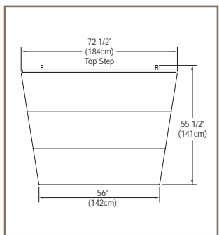
END VIEW
