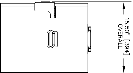
SIDE VIEW 4921 SOLID FUEL
