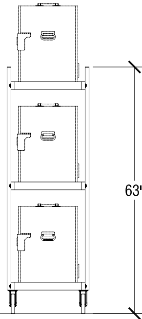
End View
