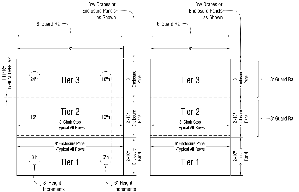
SICO Insertable Leg Riser System w/ Deck Support Legs 3' (nom.) Row Depth, Three Tier Riser
