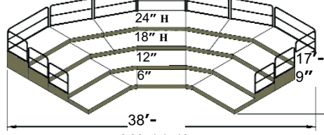
PLAN 24
