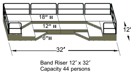
PLAN 34
