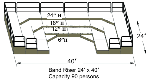
PLAN 38
