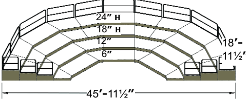
PLAN 25
