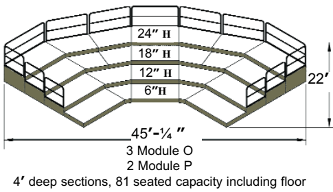
PLAN 31
