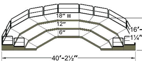
PLAN 22
