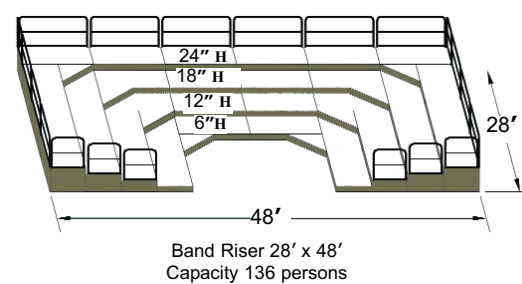
PLAN 38
