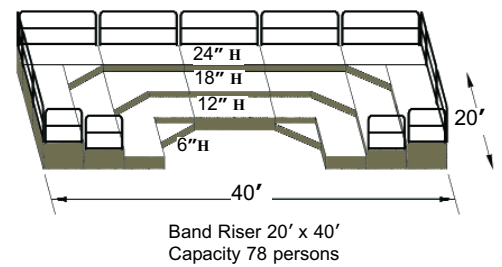
PLAN 37
