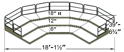
PLAN 27
