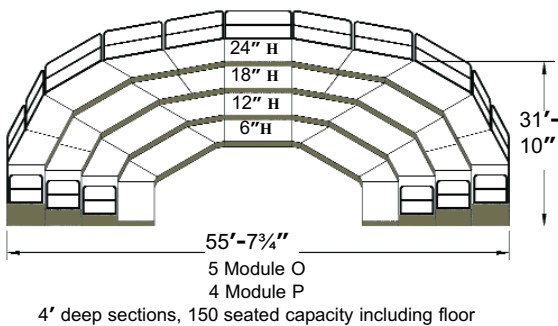
PLAN 32
