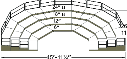
PLAN 26
