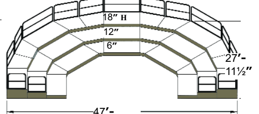
PLAN 29
