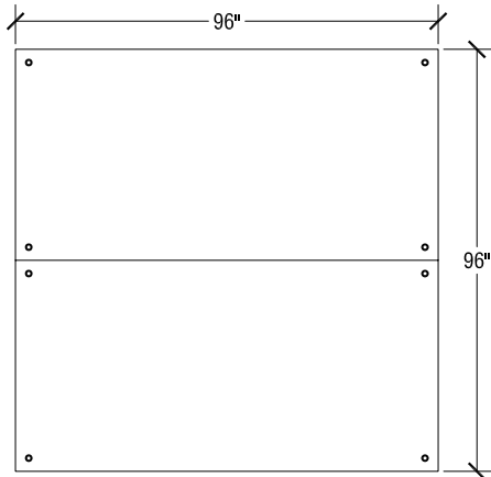
Top View (Roll-'n-Set with Two 4' x 8' Decks)
