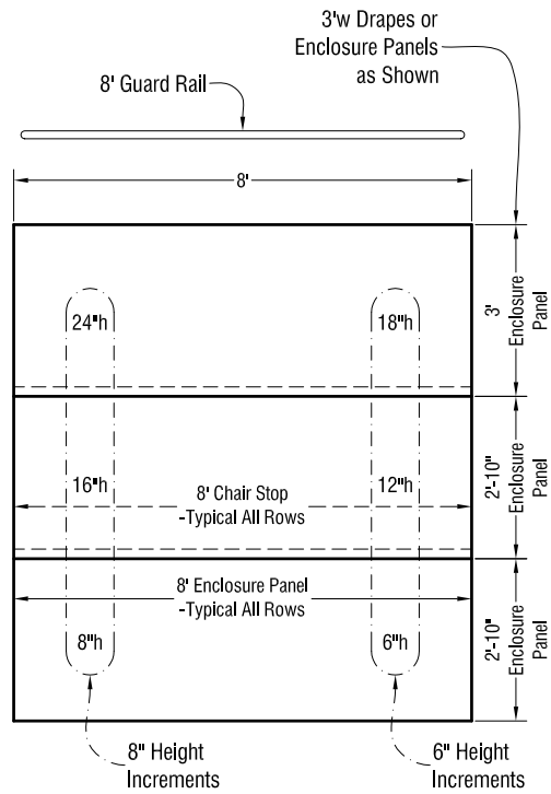
SICO X-Press Riser System 3' (nom.) Row Depth, Three Tier Riser
