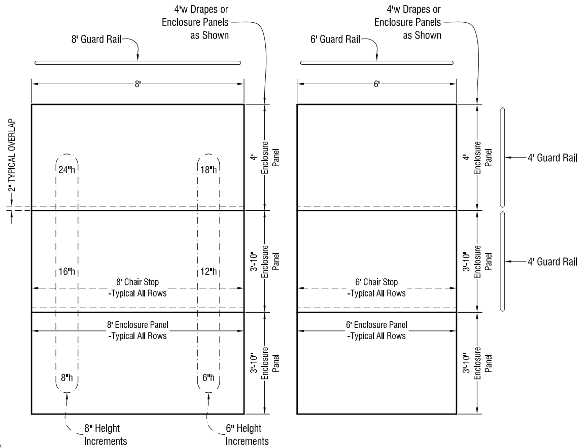
SICO X-Press Riser System 4' (nom.) Row Depth, Three Tier Riser
