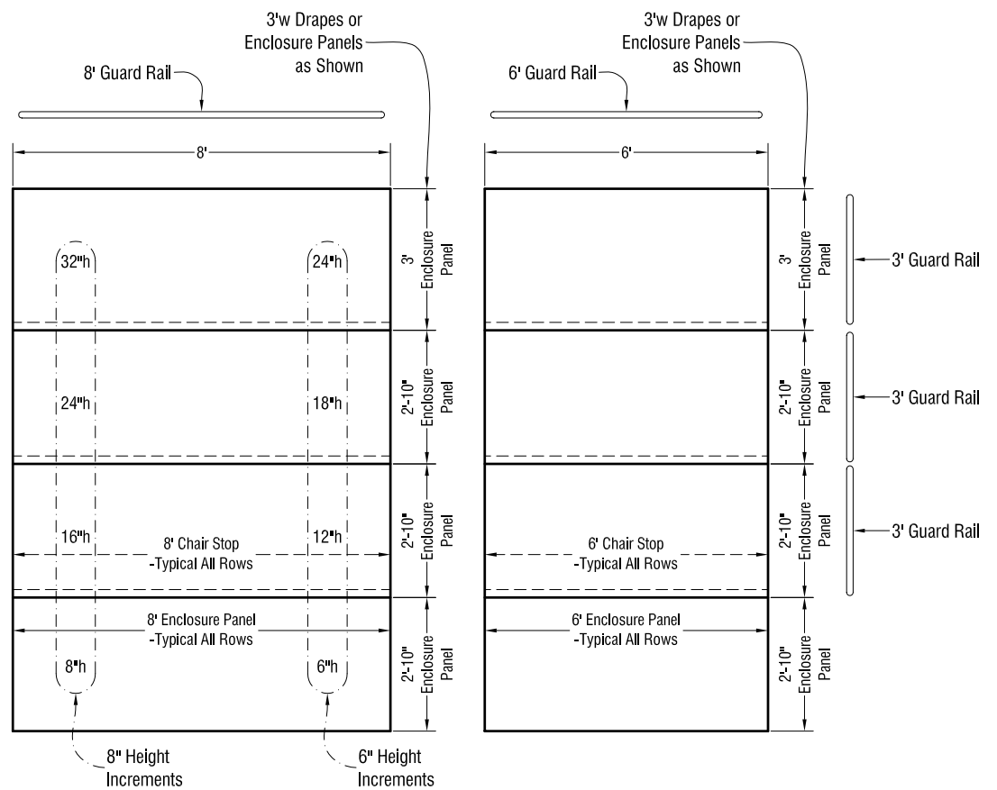
SICO X-Press Riser System 3' (nom.) Row Depth, Four Tier Riser
