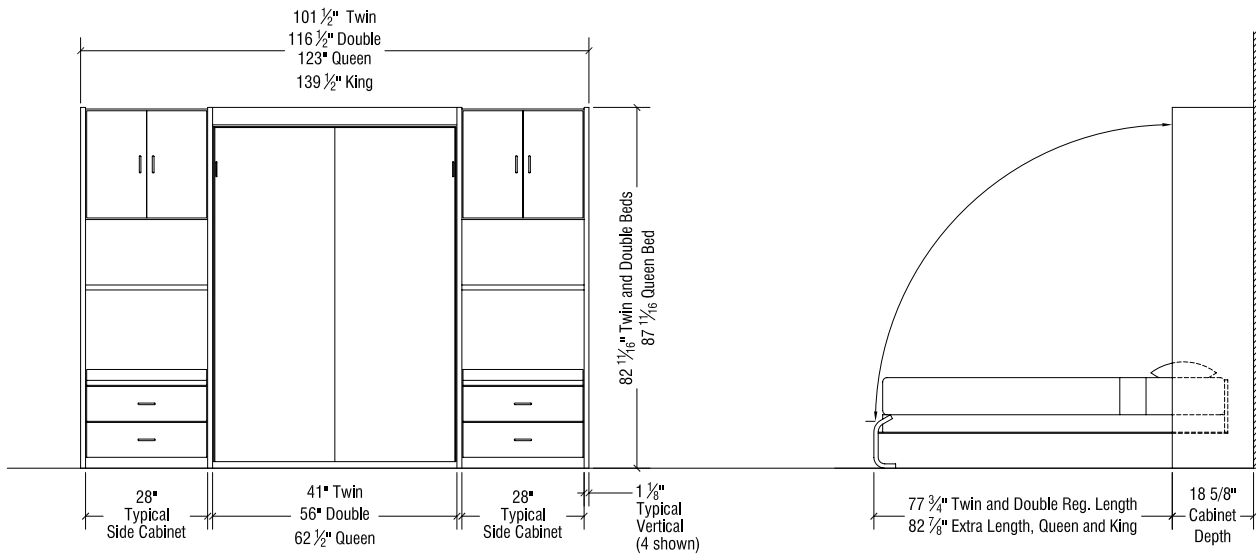
Front Elevation
