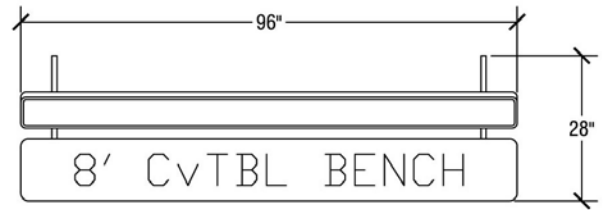
Auditorium Configuration
