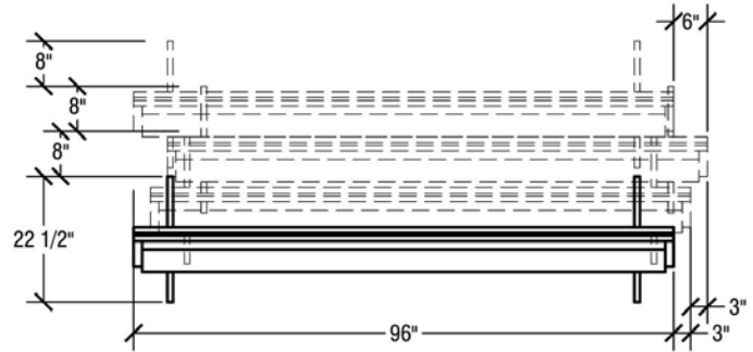
Storage Configuration
