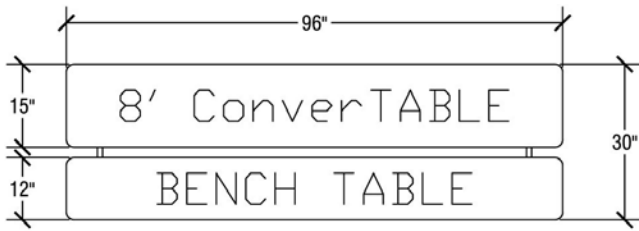
Testing Configuration
