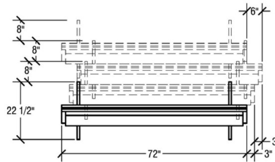
Storage Configuration
