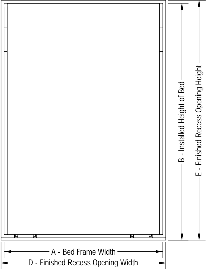
Bed Raised
