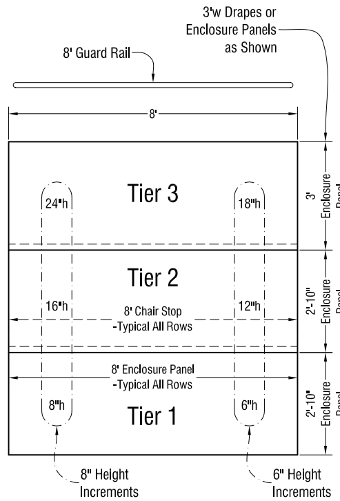
SICO X-Press Riser System 3' (nom.) Row Depth, Three Tier Riser
