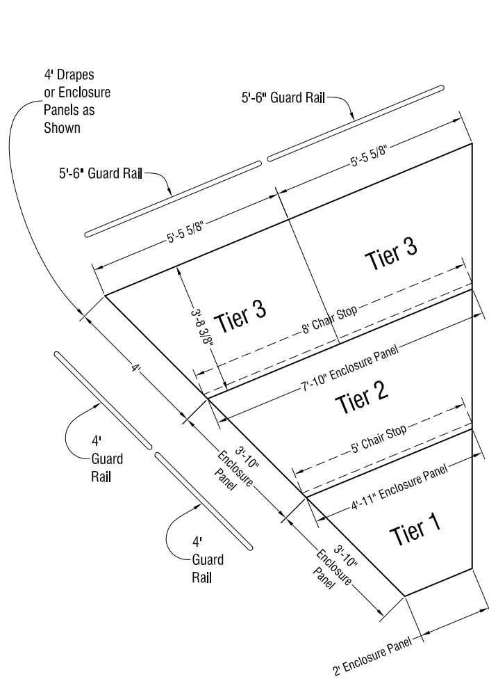
SICO X-Press Riser System 4' (nom.) Row Depth, Three Tier Riser
