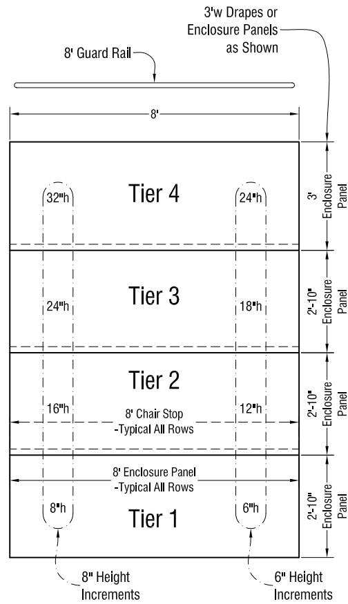
SICO X-Press Riser System 3' (nom.) Row Depth, Four Tier Riser
